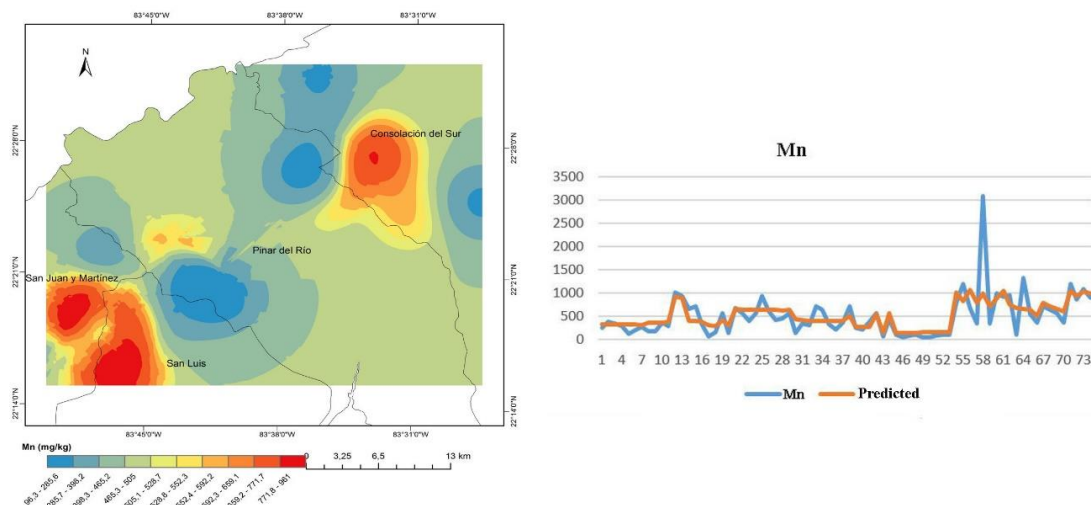
Figure 7. Spatial behavior of the Mn in the soils of the Southern Plain of Pinar del Río, Cuba
