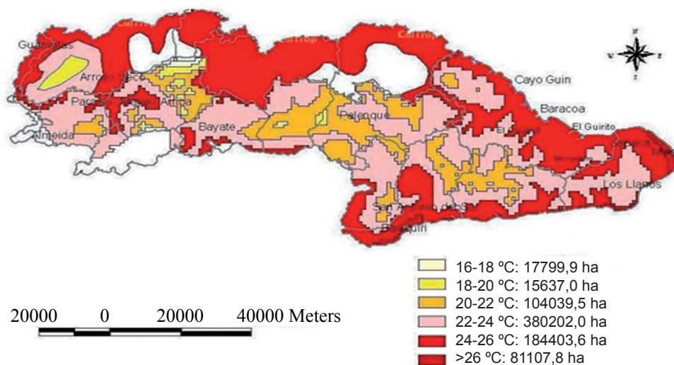
Figura 2. Map showing mean annual temperatures at the Nipe-Sagua-Baracoa mountain range
