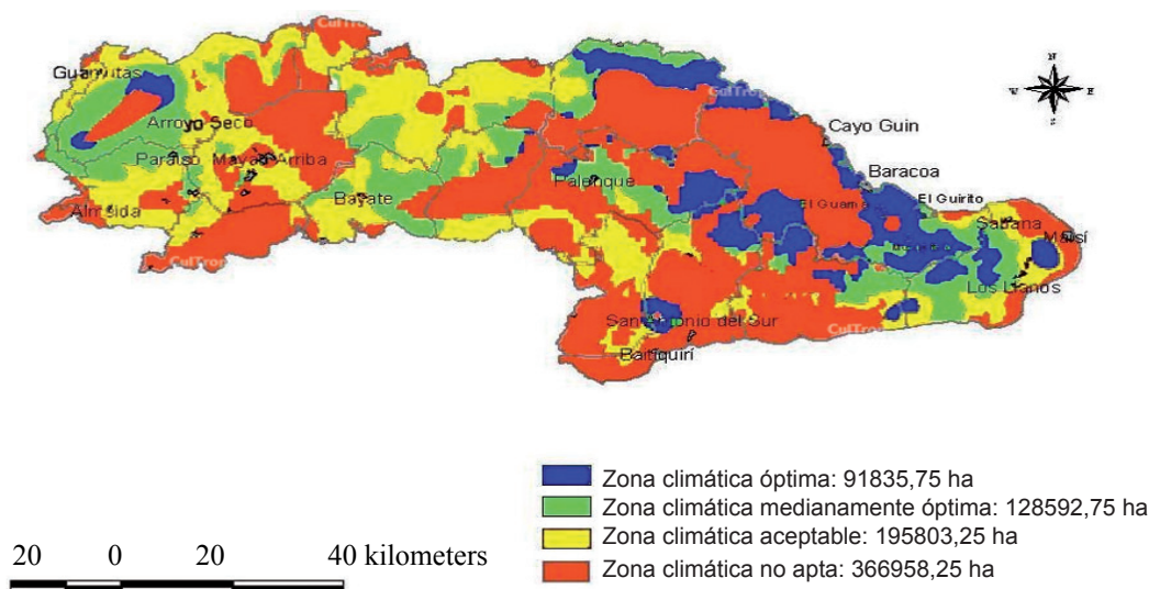
Figura 3. Map with climatic regions to grow cocoa in the Nipe-Sagua-Baracoa mountain range
