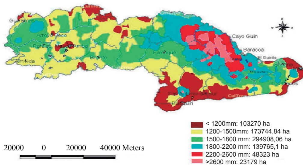
Figure 1. Mean annual rainfall in the Nipe-Sagua-Baracoa mountain range
